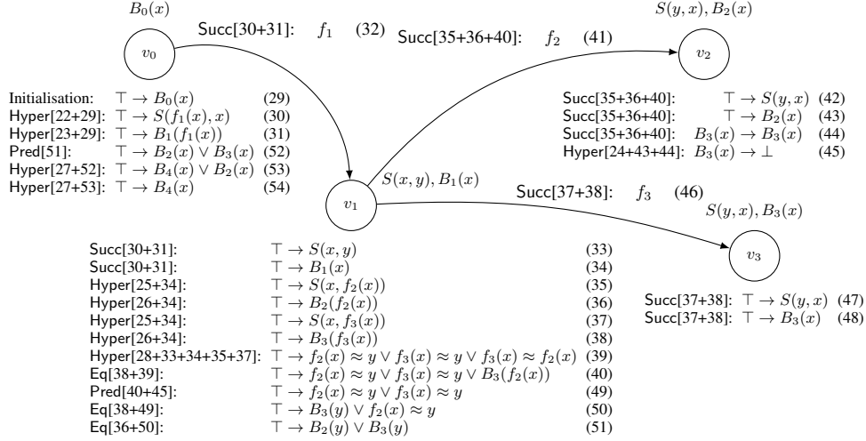
Figure 2: Challenges in Extending the Consequence-Based Framework to \mathcal{ALCHIQ}
