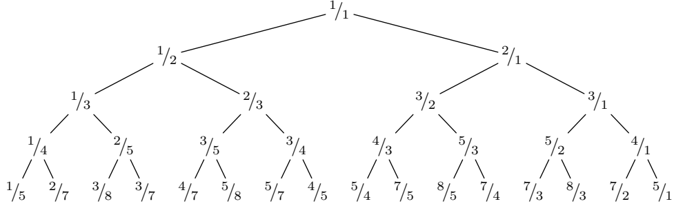
Fig. 3. The Stern-Brocot tree
