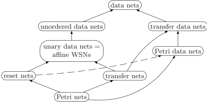
Fig. 1. Inclusions among classes of data nets
