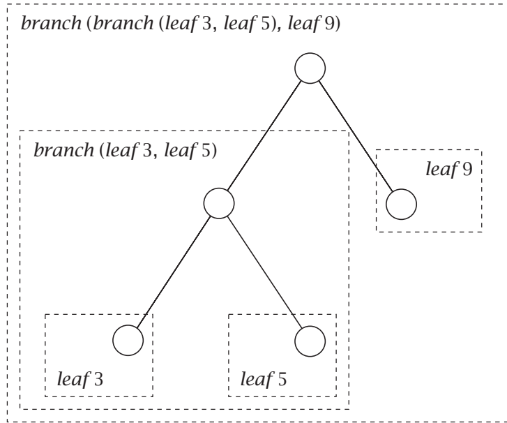
Figure 10.2 A binary tree
